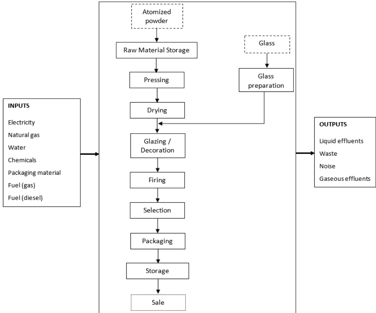
Figure 1 – Flowchart of the manufacturing production process.
